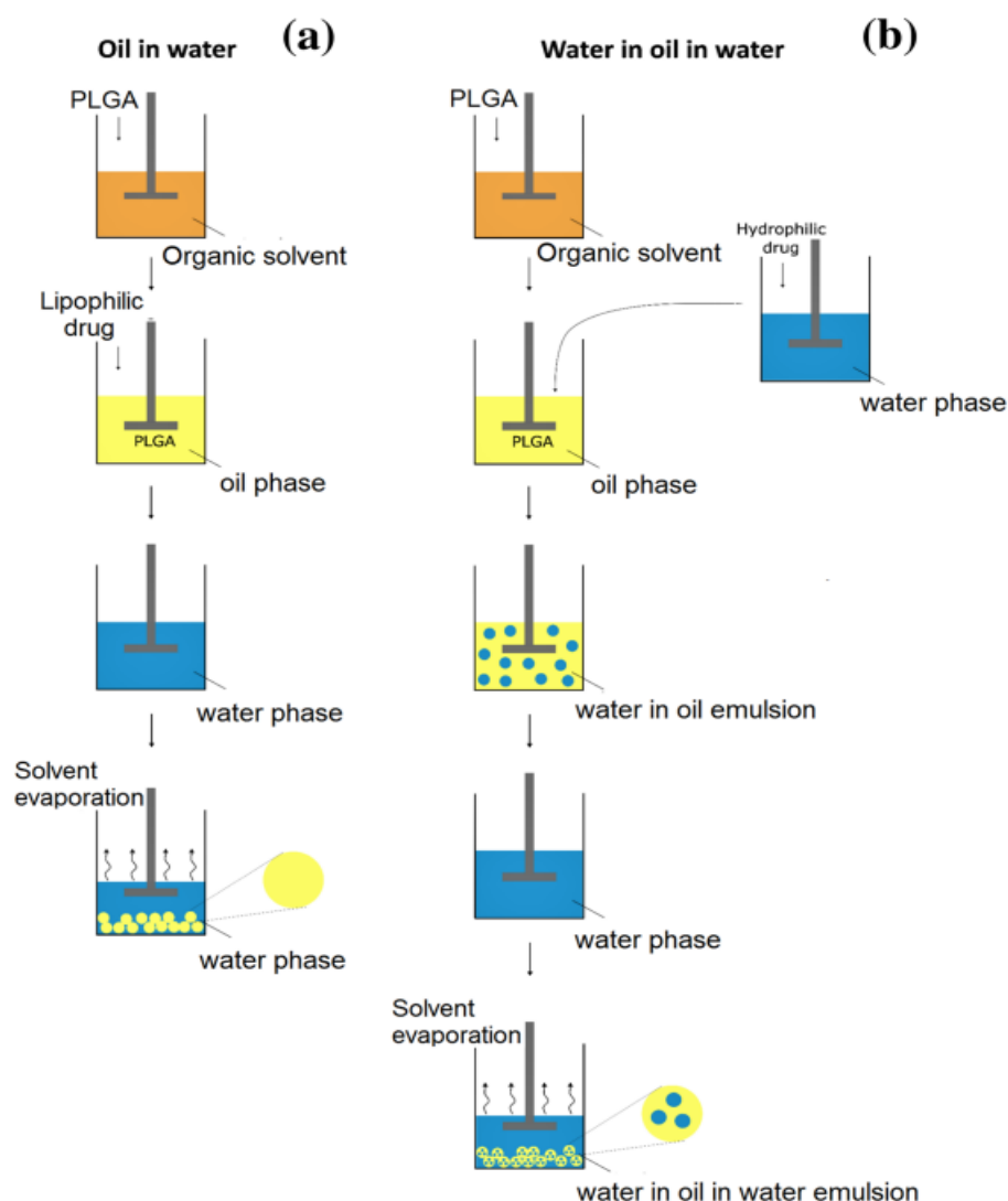
Figure 3: Schematic representation of emulsion techniques: O/W single emulsion method (a) and W/O/W double emulsion (b). [55]
