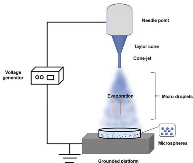
Figure 5. Schematic of the electrospray process. [95]
